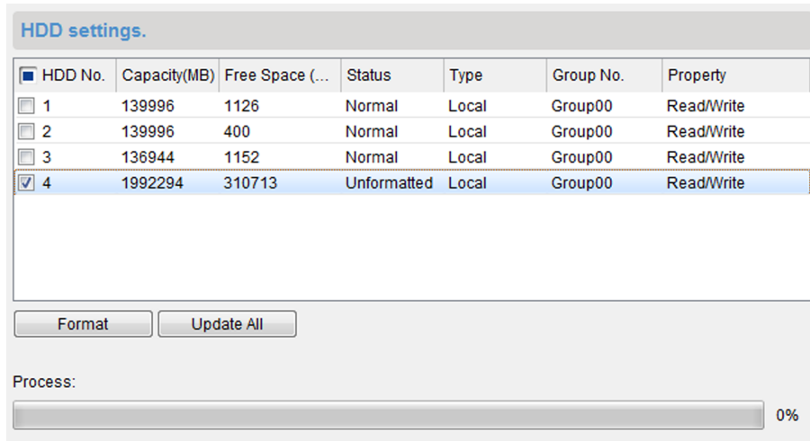
Figure 6-1 HDD Formatting
